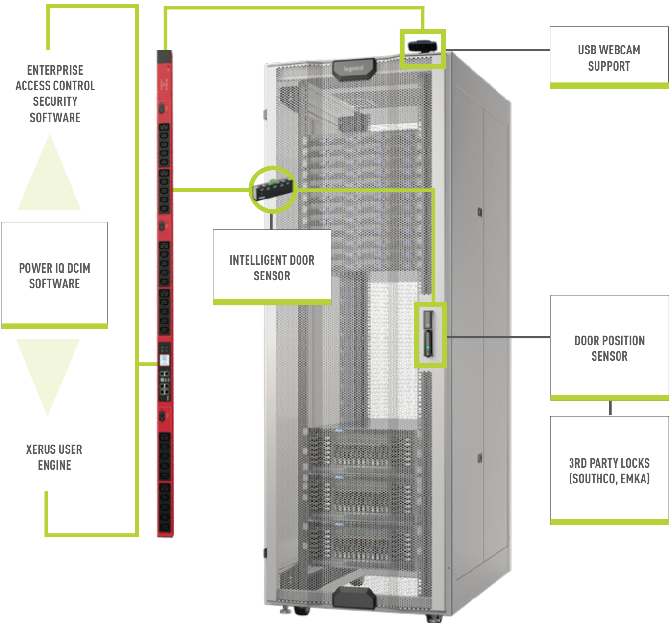
PX INTELLIGENT RACK PDU / SRC SMART RACK CONTROLLER
